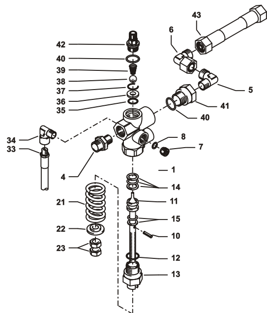
Safety valve for heating coil (Adjustment must be approx. 15% above the operating pressure)
