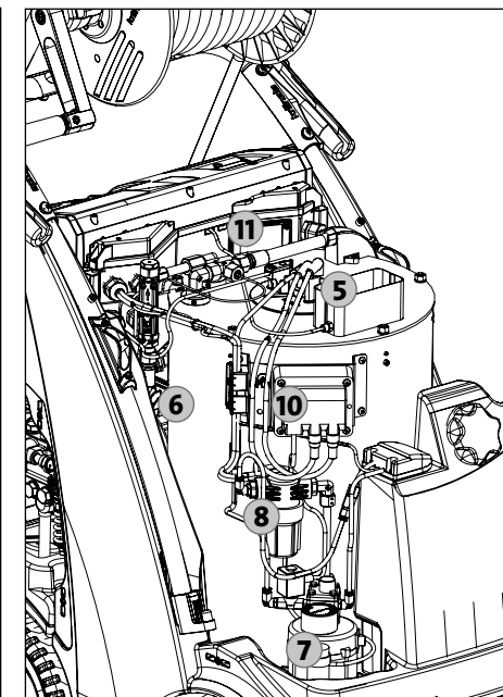
Large cap removed
