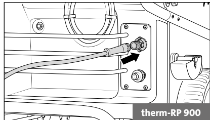
therm-RP 900
